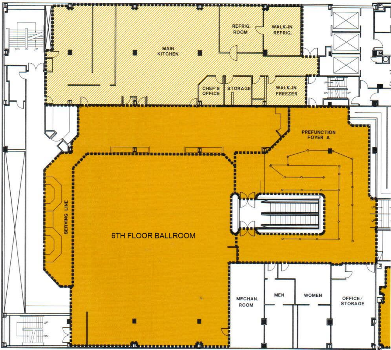
ENLARGED FLOOR PLAN - PART A
